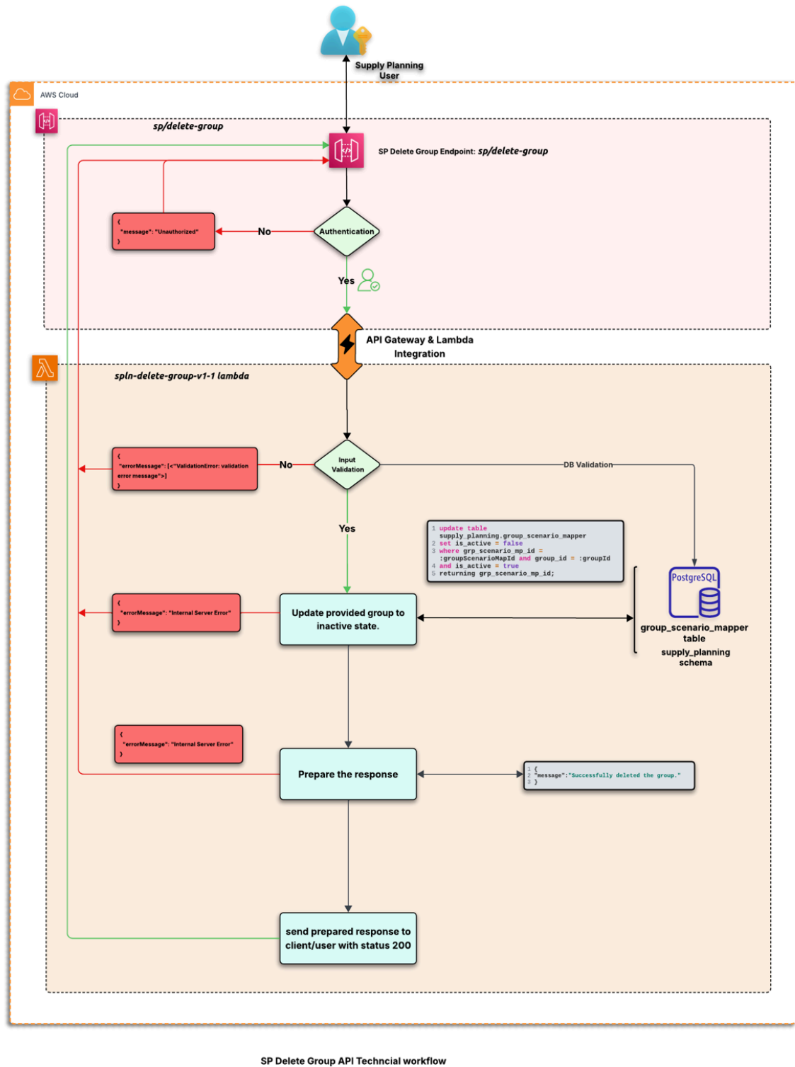
SP Delete Group API Technical workflow
